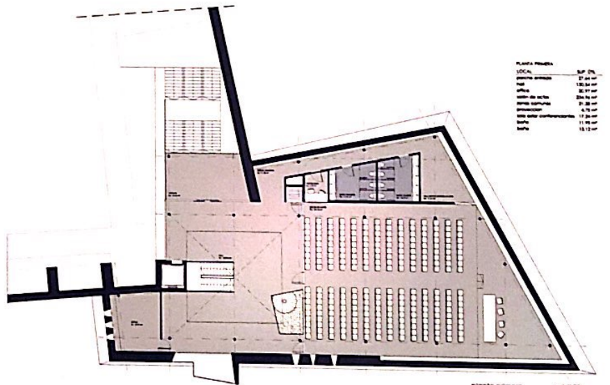
piano prima • 1/150
